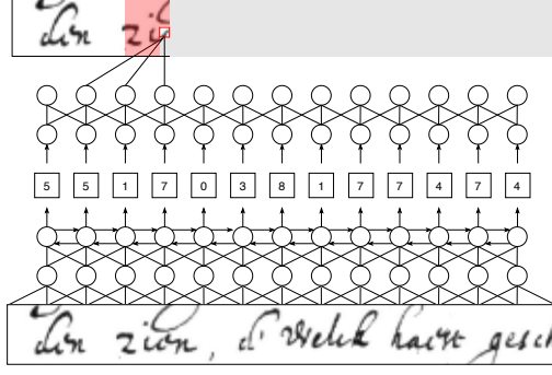
Figure 1: Model architecture. The encoder combines convolutional and recurrent layers and extracts a sequence of embeddings, which are quantized and used as conditioning of an autoregressive PixelCNN decoder. The decoder produces consistent samples, by filling in the details missing in the low-bandwidth encoding with information from the autoregressive path.
