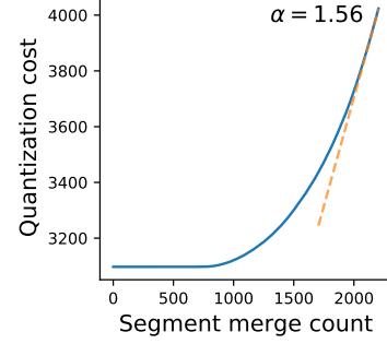
Figure 2: The Lagrange multiplier \alpha of a constraint corresponds to increase of the objective function for an infinitesimal change in the constraint.
