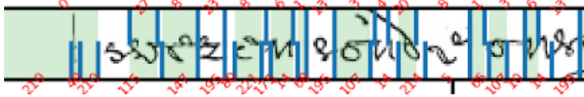
Figure 3: Unsupervised segmentations obtained with the proposed criterion. The top half shows ground truth segmentation (vertical bars) and character codes. The bottom half shows model segmentation and prototype indices (out of 256). Green-shaded columns are properly classified by a many-to-one mapping of prototype to characters. For instance, we can see the model learned to properly delineate and recognize the character “o”, consistently assigning it to cluster 107.
